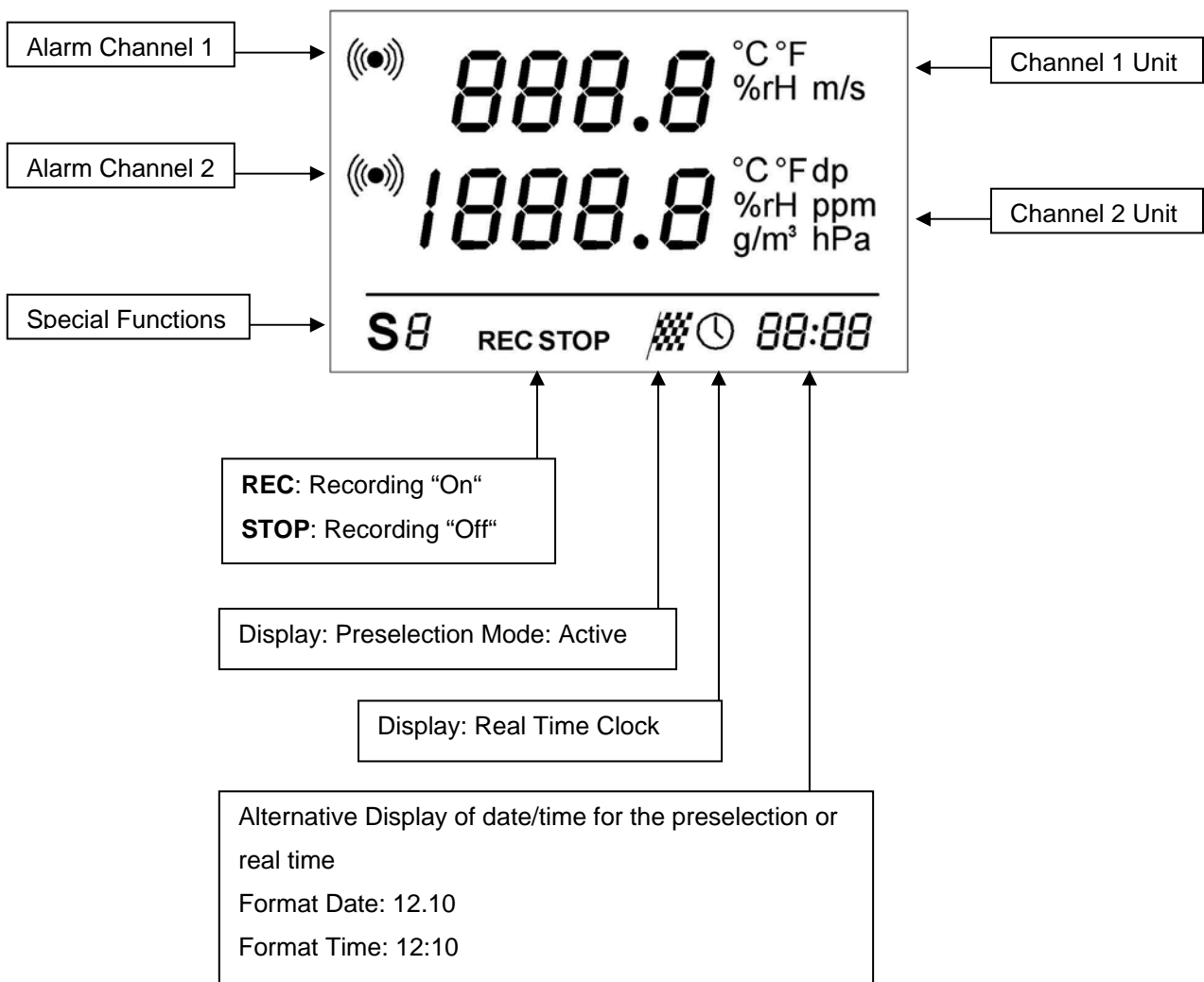
Illustration: HUMLOG 10 Display Elements
